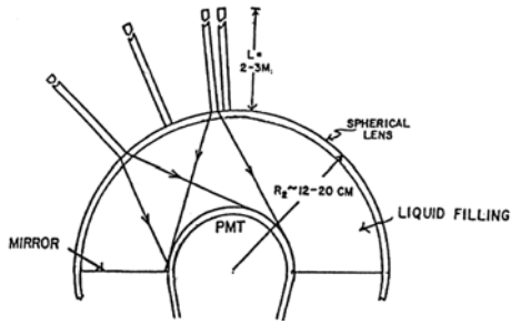
Fig. 5. The Sea-Urchin (figure taken from [Roberts 1992]). See text for explanation.
