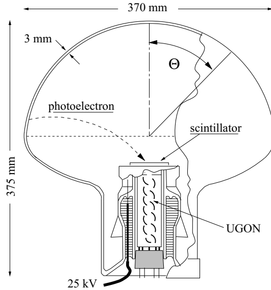
Fig. 8. The QUASAR-370 phototube.
