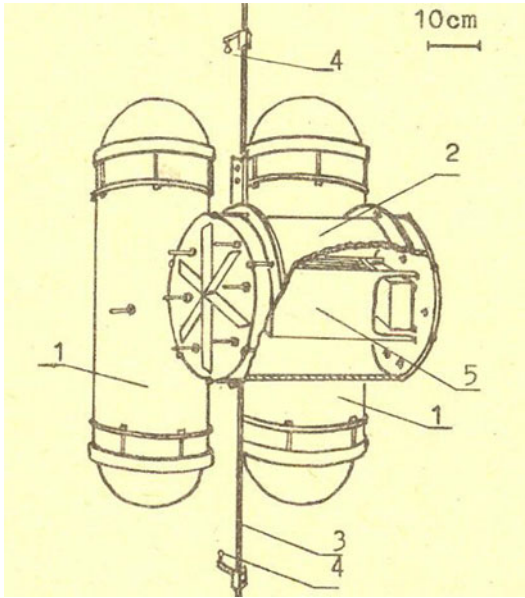
Fig. 7. A “ svjaska ” (Russian for “bundle”) as used in GIRLANDA-86 for the monopole search, with 4 PMTs in 2 cylinders (1) covered by hemispheric plexiglass caps. The “backpack” module (2) contains electronics (5). Calibration LEDs (4) are fixed at the geophysical cable (3).
