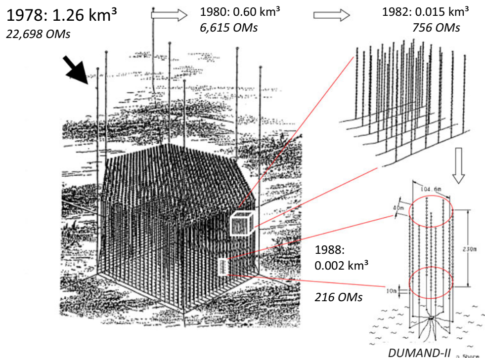
Fig. 4. The originally conceived DUMAND cubic kilometre detector and the phased downgrading to the 1988 plan for a first-generation underwater neutrino telescope DUMAND-II. See text for explanations.
